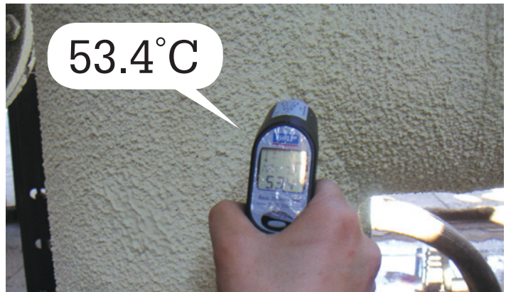
Temperature after HPC® Coating application was 128.12°F
